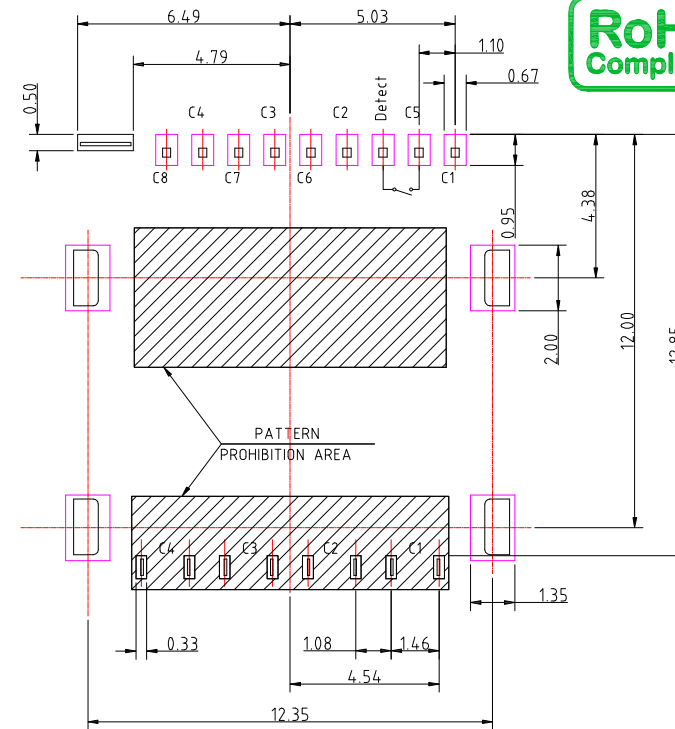
PCB LAYOYT
